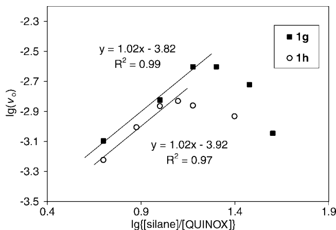
Figure 2. Reaction order in 2 .
